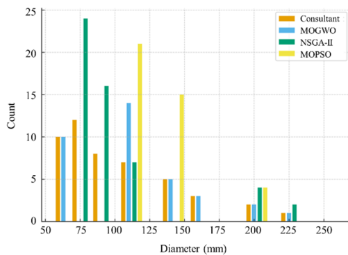
Figure 5. Pipe Diameter Distribution
