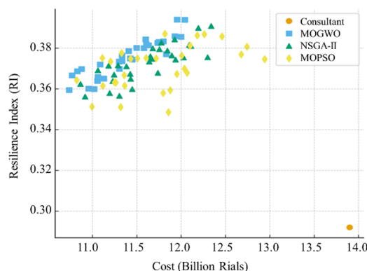
Figure 2. Pareto front analysis
