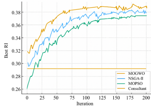
Figure 4. RI convergence analysis
