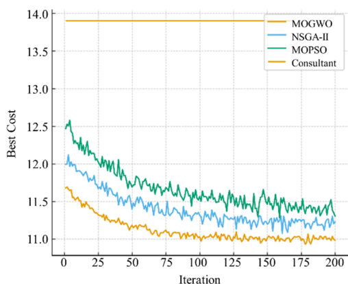
Figure 3. Cost convergence analysis
