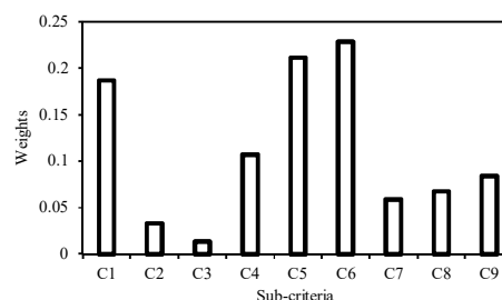
Figure 2. Final weight of sub-criteria from Entropy-Shannon method
