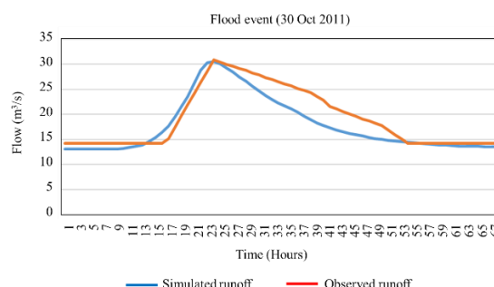
Figure 7. Hydrograph of validation of the model built in the Hablehroud basin
