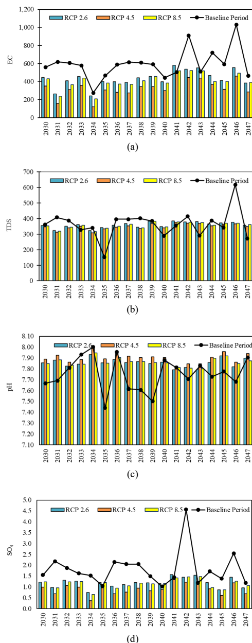
Figure 1. Variation of parameters (a) EC, (b) TDS, (c) pH, and (d) SO_4 in the future period under different scenarios
