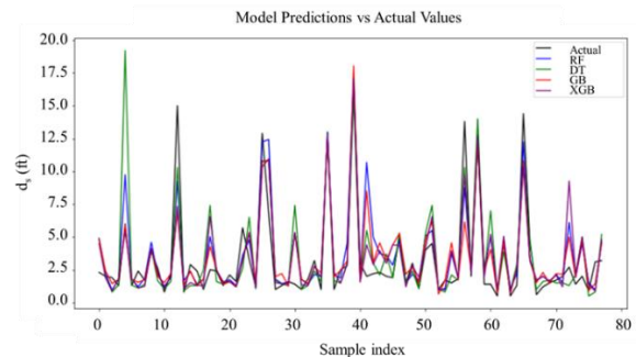
Figure 5. Comparison of calculated scour height values by different models with actual scour values
