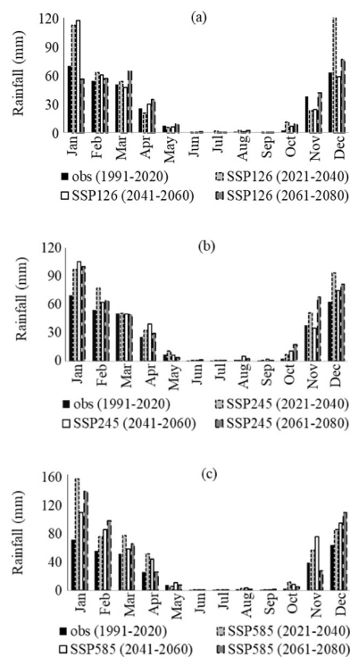
Figure 4. Changes in monthly rainfall in baseline period (obs) and three future 20-year periods under scenarios (a) SSP126, (b) SSP245 and (c) SSP585 in Shiraz
