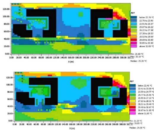
Figure 12. PET images in summer (Celsius)
