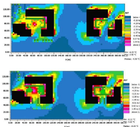
Figure 12. PET images in winter (Celsius)
