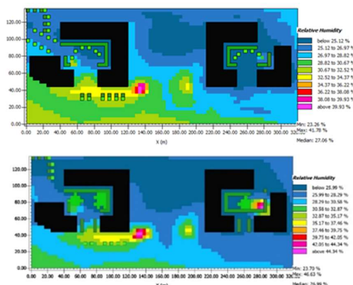
Figure 6. Summer relative humidity images (percentage)
