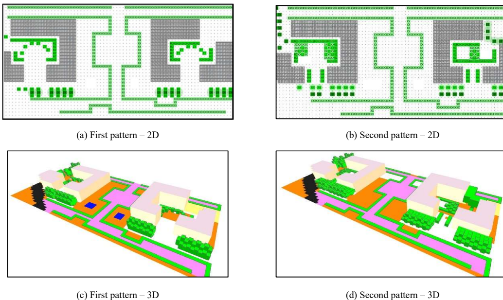
Figure 1. Modeled patterns (2D and 3D) in ENVI-met software
