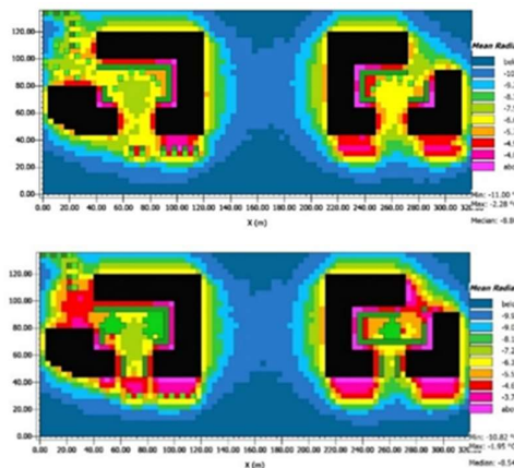
Figure 9. Average winter radiant temperature images (Celsius)
